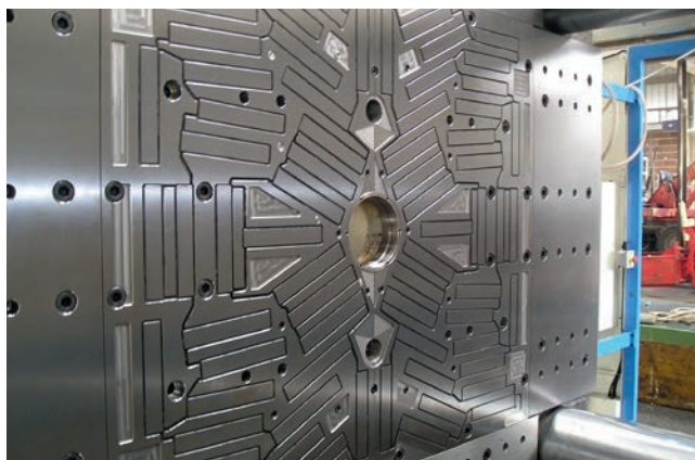
Pressmag HP on a 32000 kN (3200 t) machine
